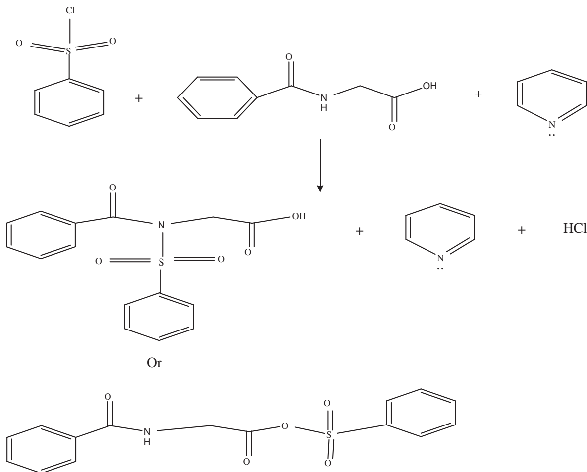
Figure 4 Chemical equation of color test method.
